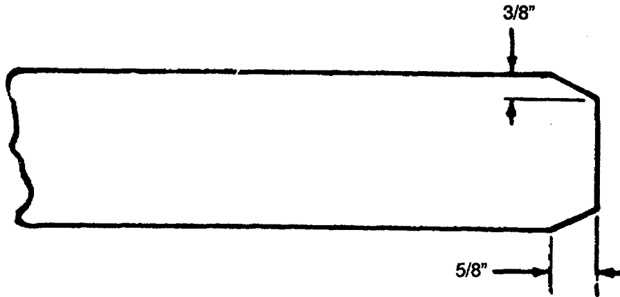
Figure 2-25. Trim Details for Lateral Strap End Without Adapter
