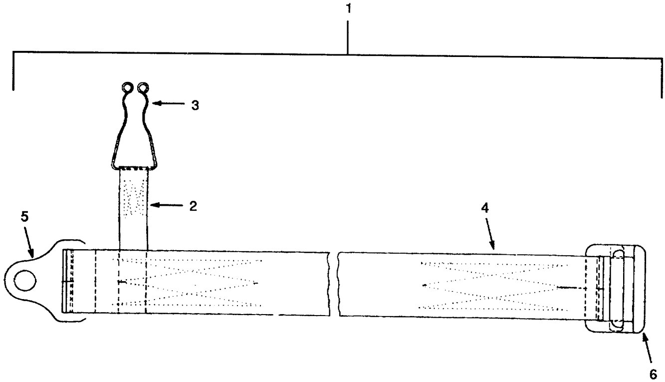
Figure C-4. Strap, Quick Release, Fixed
