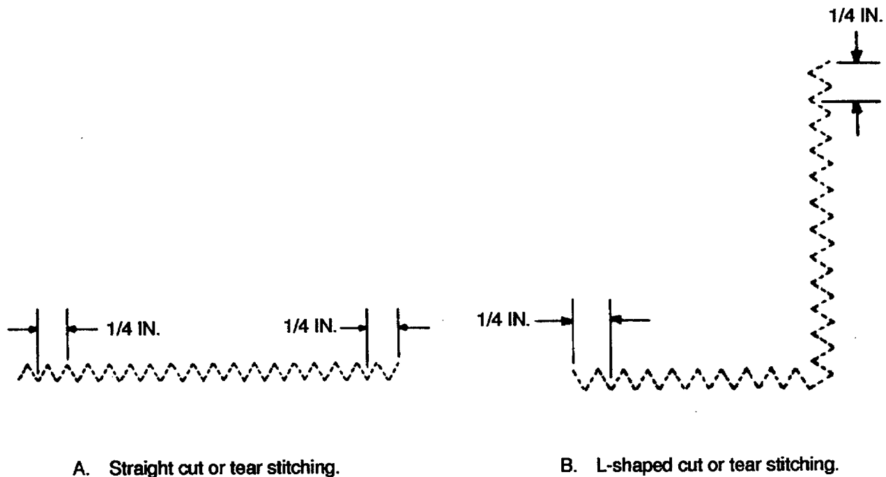
Figure 2-3. Repair Method Using a Zigzag Sewing Machine
