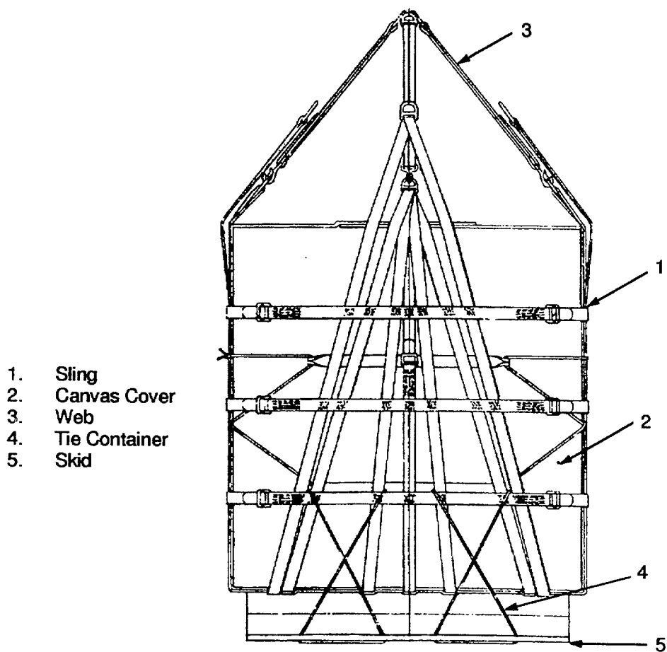
Figure 1-9. A-23 Cargo Bag
