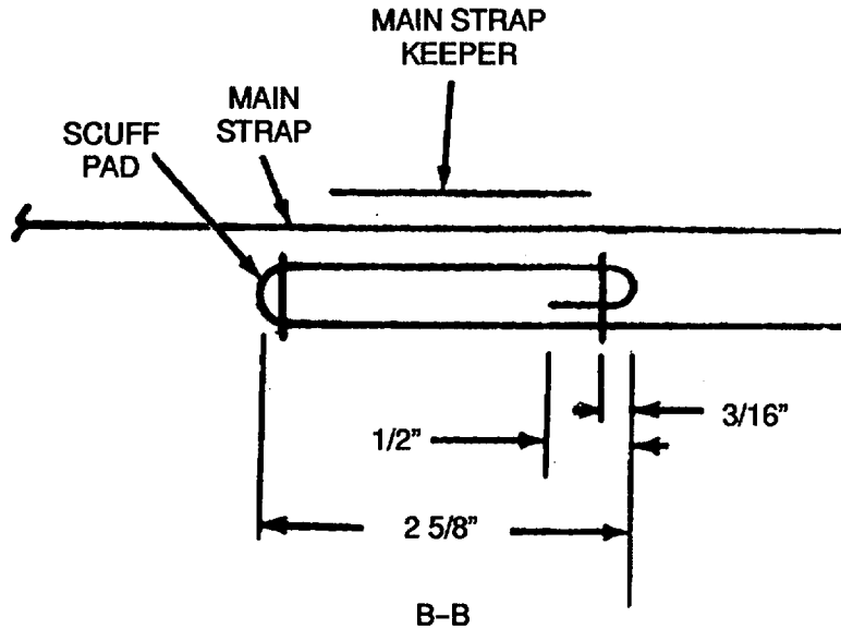
Figure 2-18. Main Strap Keeper Sewing Details
