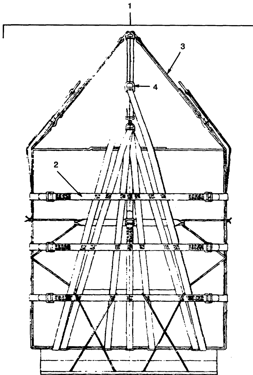
Figure C-13. A-23 Cargo Bag
