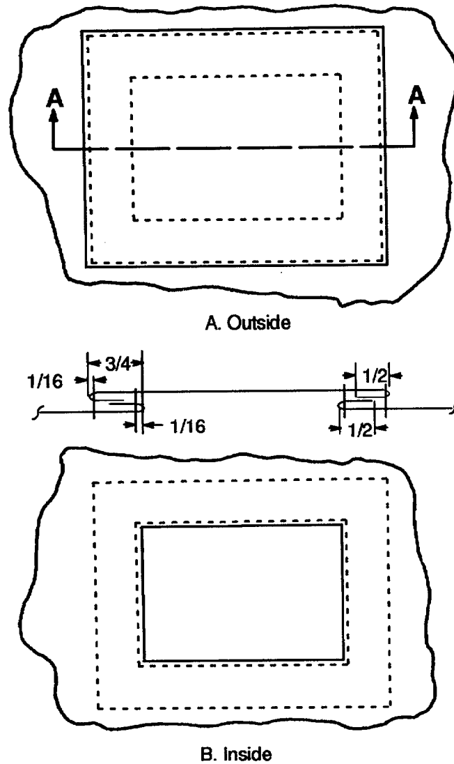
Figure 2-13. Patching Details for Cover
