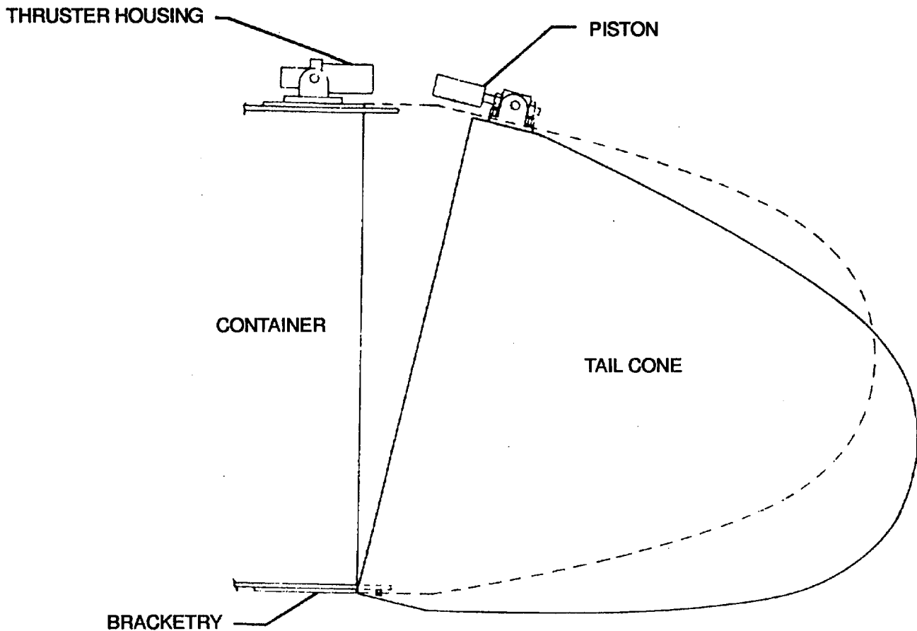
Figure 2-37. Tail Cone Assembly
