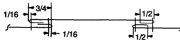
Figure 2-16. Patching Details for Scuff Pad
