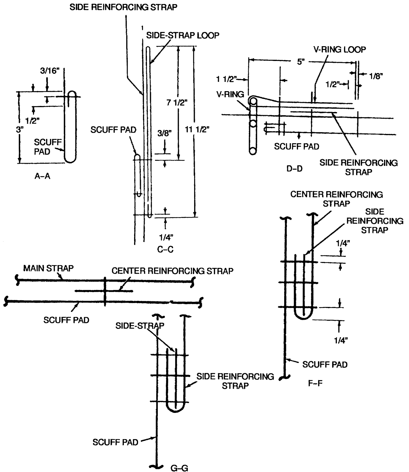
Figure 2-19. Sewing Details on A-21 Cargo Bag Sling Straps and Loops
