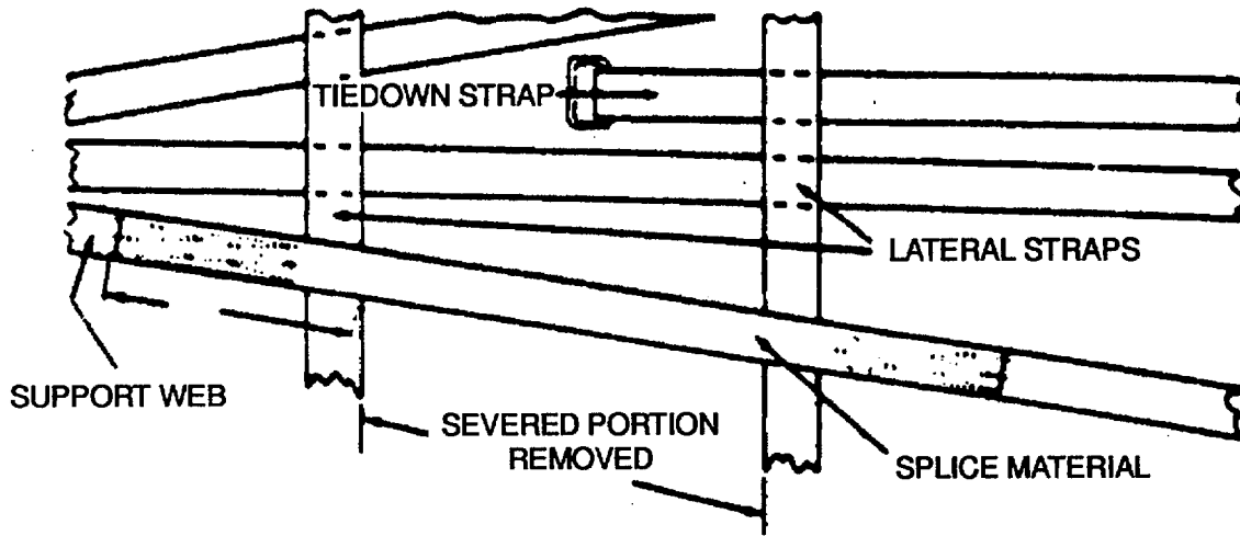
Figure 2-24. Splicing Details for a Severed Support Web
