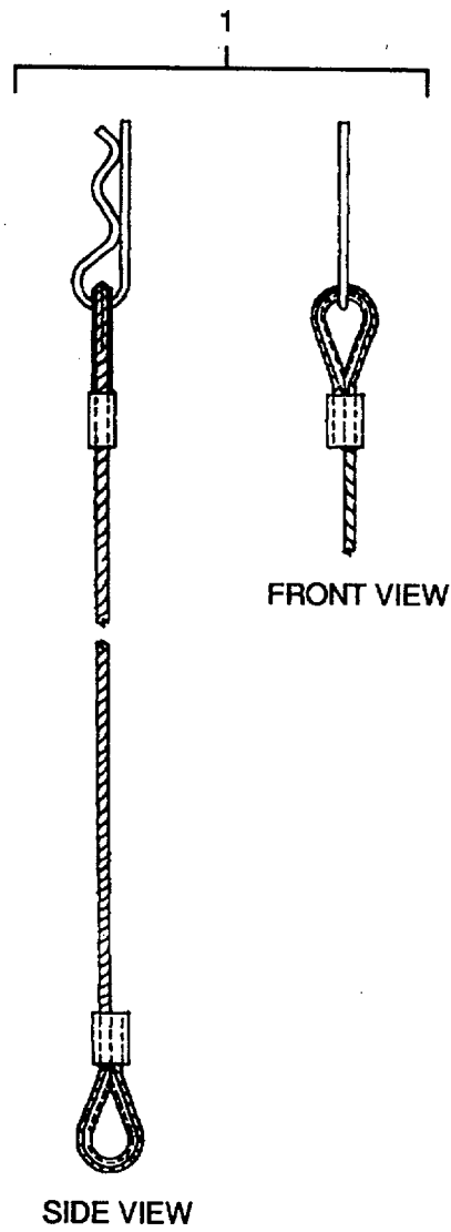
Figure C-22. Cable Assembly, Parachute Release
