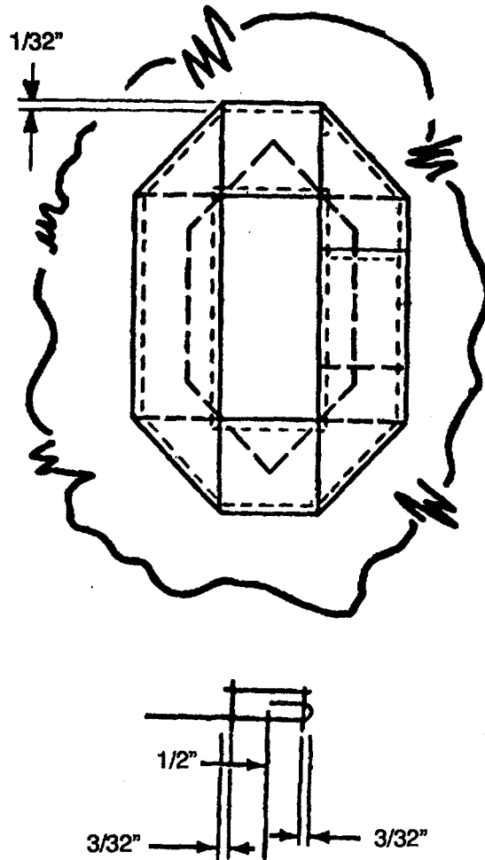
Figure 2-17. Scuff Pad V-Ring Hole Reinforcement Details
