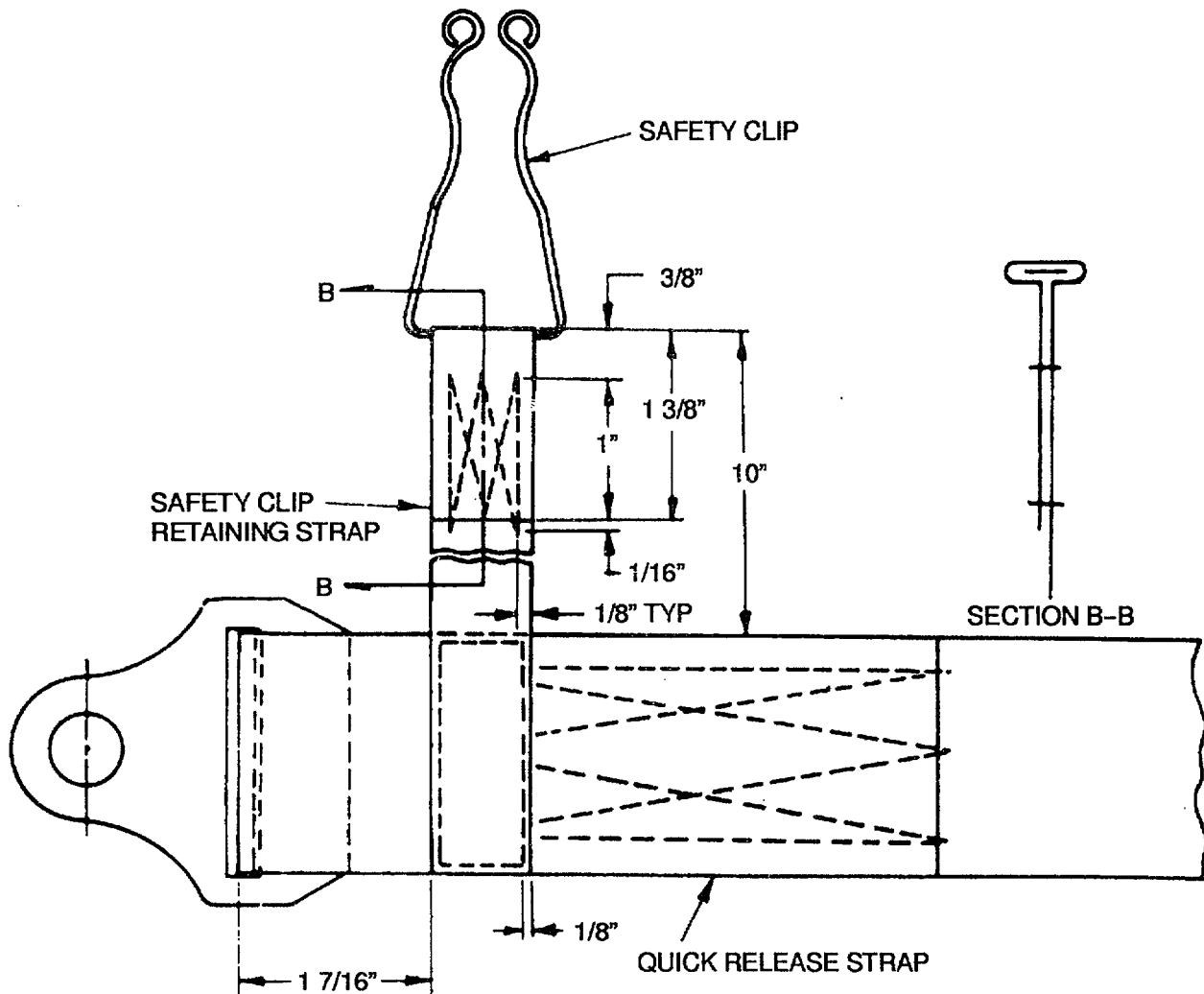
Figure 2-20. Fabrication and Installation Details of the Safety Clip Retaining Straps
