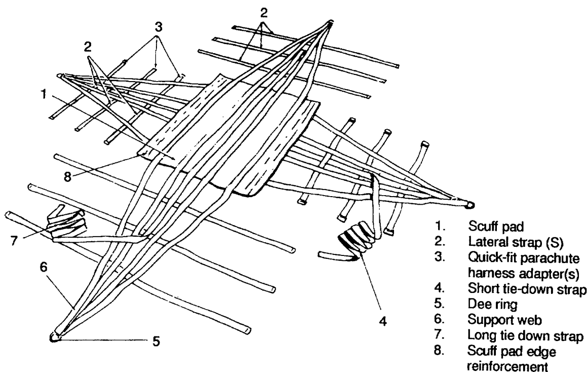
Figure 1-6. Sling Assembly
