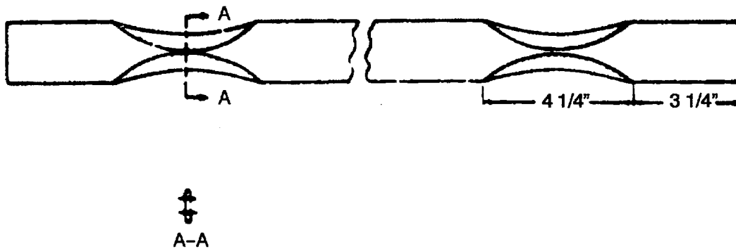
Figure 2-21. Fabrication Details of A-22 Cargo Bag Cover Lacing Loop Strap
