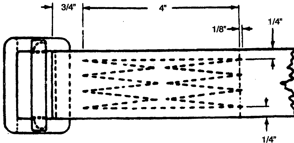
Figure 2-26. Quick-fit Adapter Installation Details
