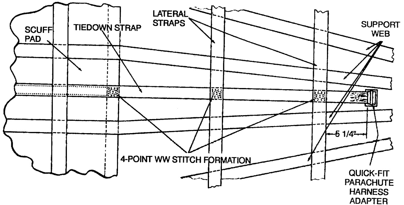
Figure 2-27. Tie-down Strap Installation Details
