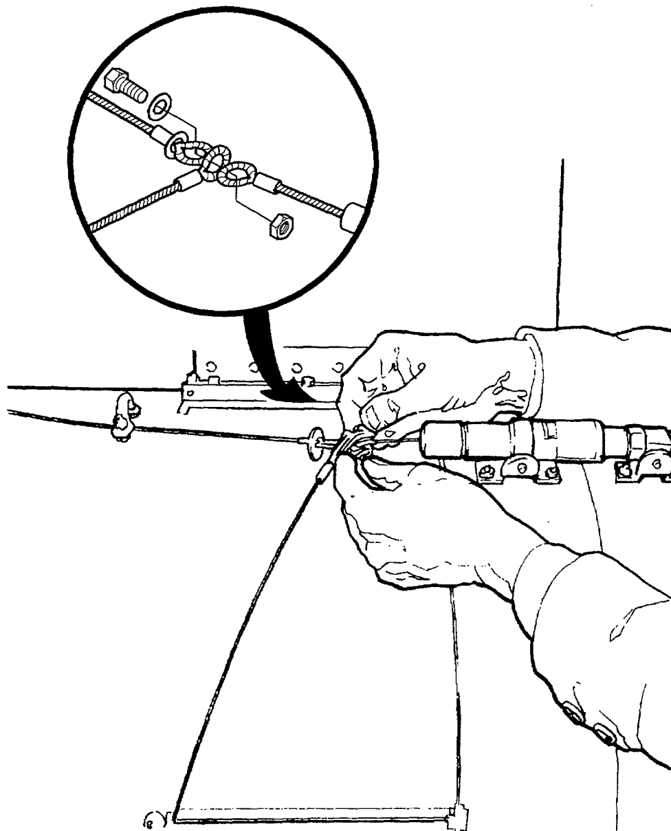
Figure 2-29. Parachute Cable Release Assembly
