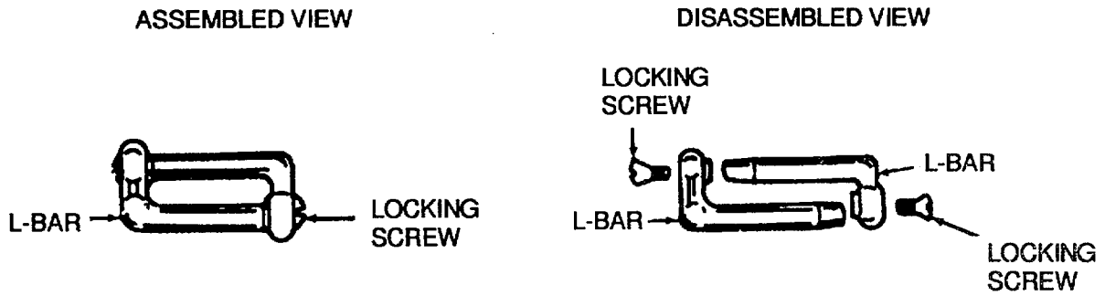
A. The L-bar Parachute Connector Link Assembly.
