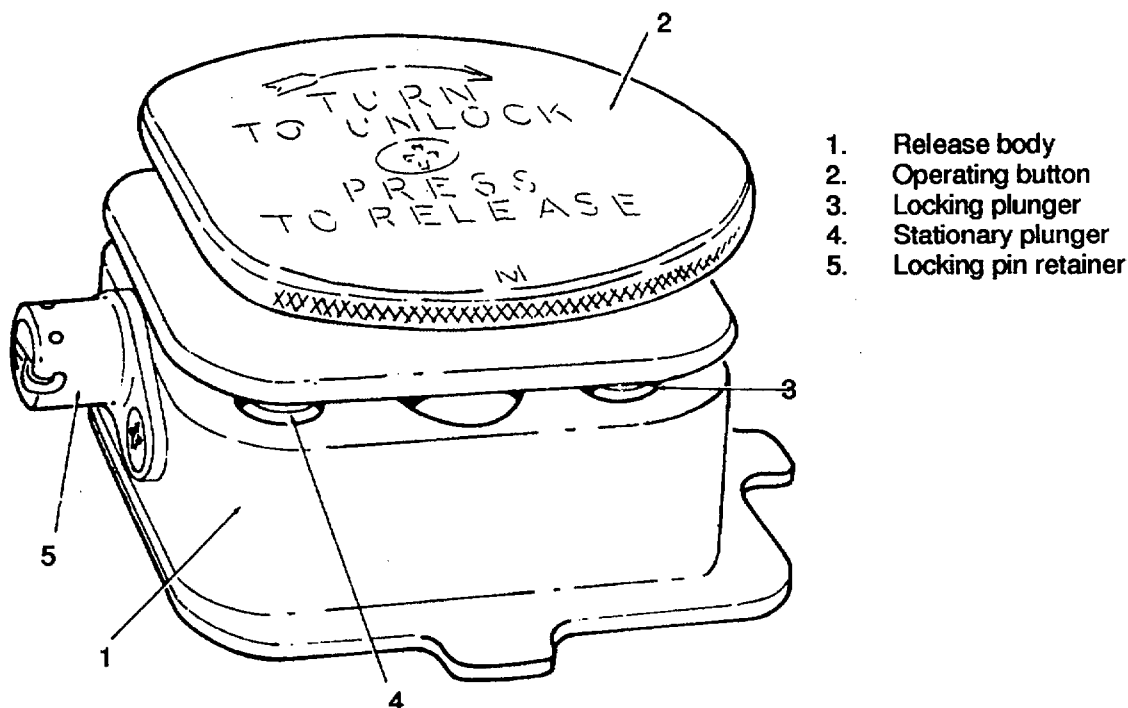
Figure 1.4. Quick Release Assembly
