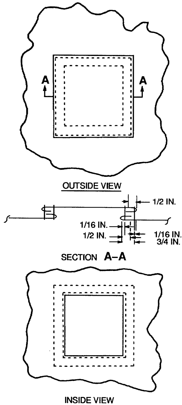
Figure 24. Basic Patch Application to Other Airdrop Equipment
