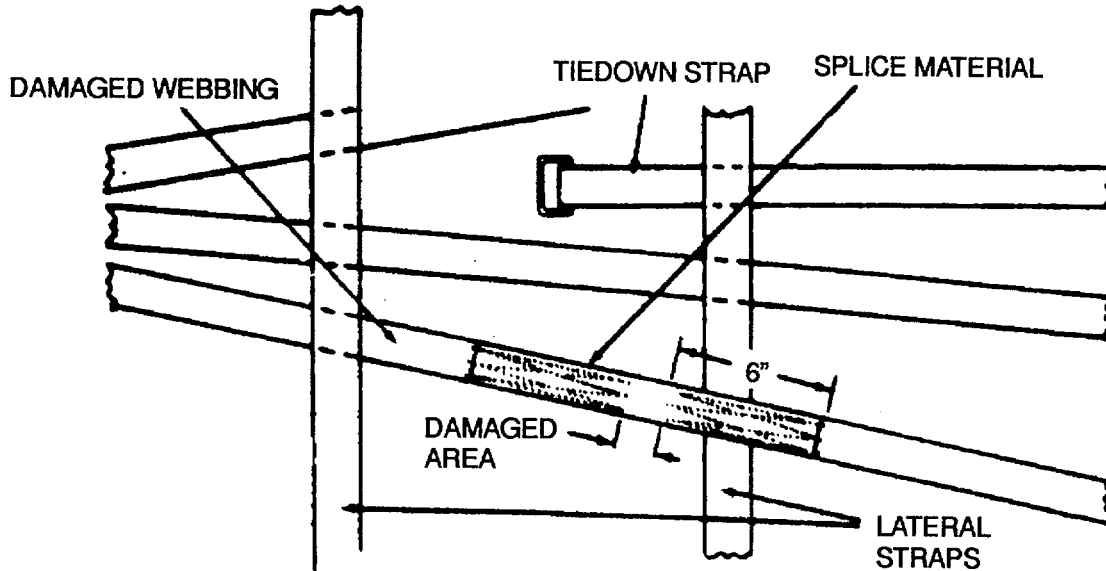
Figure 2-23. Splicing Details for a Damaged Support Web
