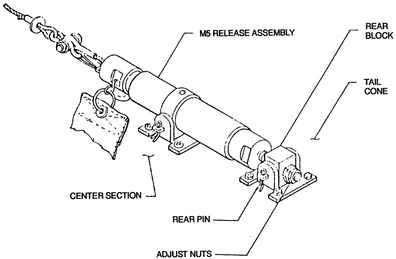
Figure 2-32. M5 Cartridge-Actuated Release Assembly
