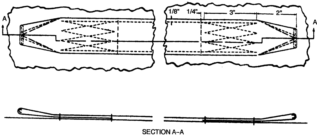
Figure 2-22. Installing Cover Lacing Loop Strap
