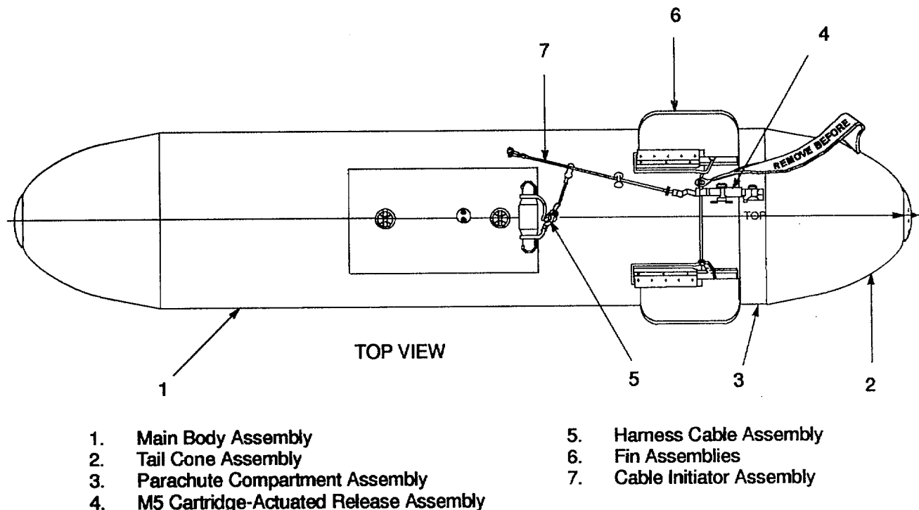
Figure 1-10. CTU-2/A Cargo Capsule
